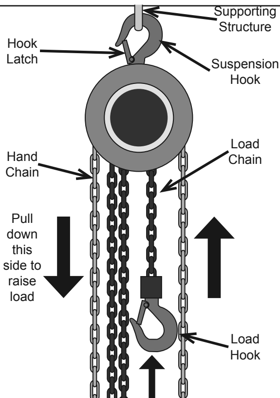
Figure E: To Raise the Load
