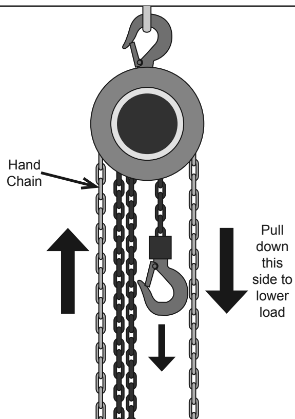
Figure F: To Lower the Load
