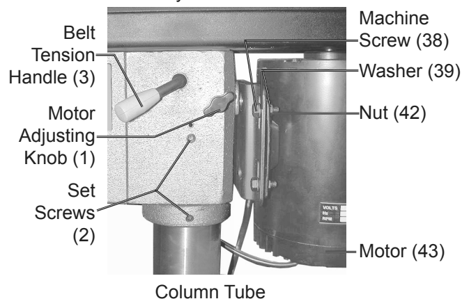
Head Assembly
