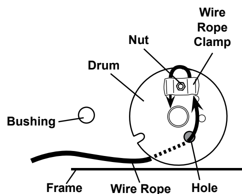
Figure J: Wire Rope Replacement
