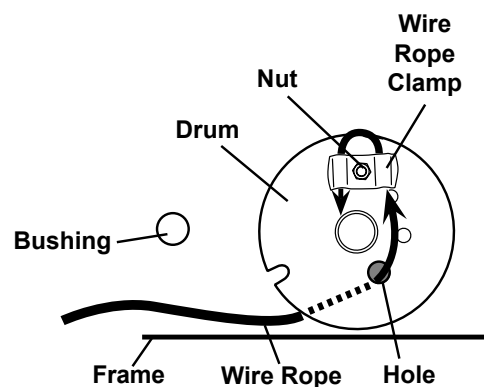
Figure I: Wire Rope Replacement
