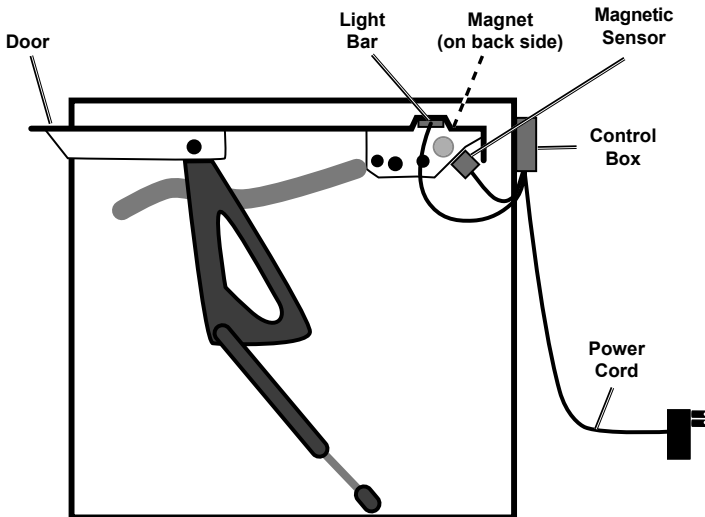
Inside Cabinet - Side View
