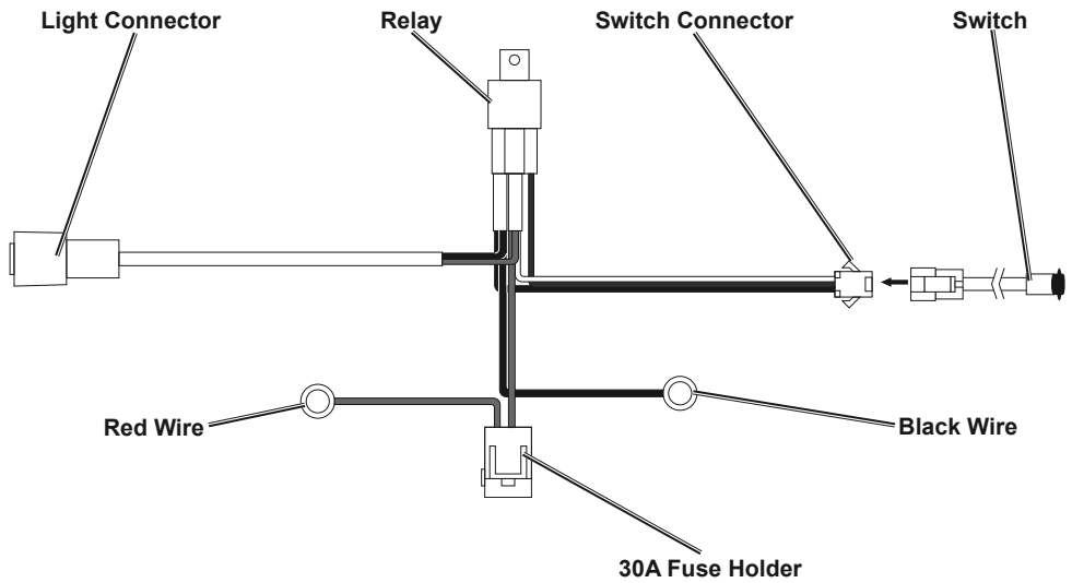
Figure B: Wiring Harness Connections
