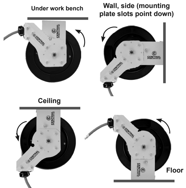
Figure C: Mounting examples.
