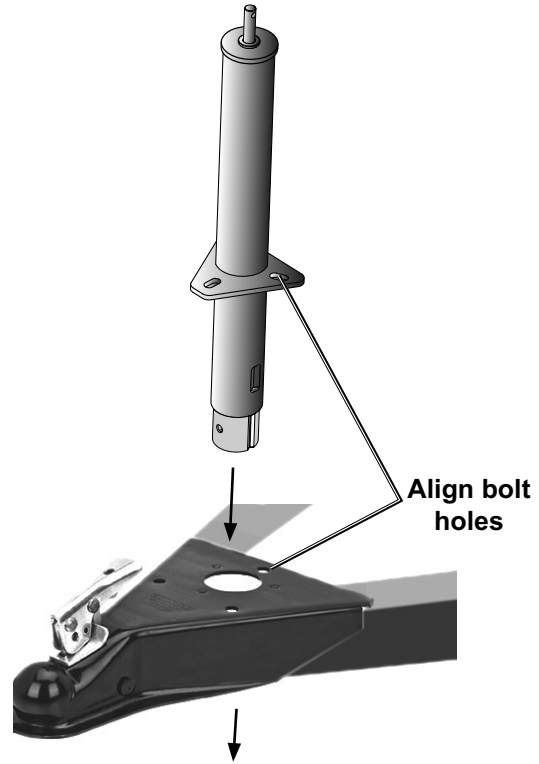
Figure A: Inserting Trailer Jack into Coupler
