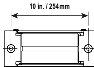
Figure B: Fairlead Mounting Dimensions
