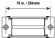
Figure B: Fairlead Mounting Dimensions
