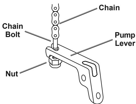
Chain Attachment Detail
