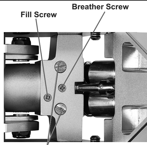
Figure A: Hydraulic Unit
