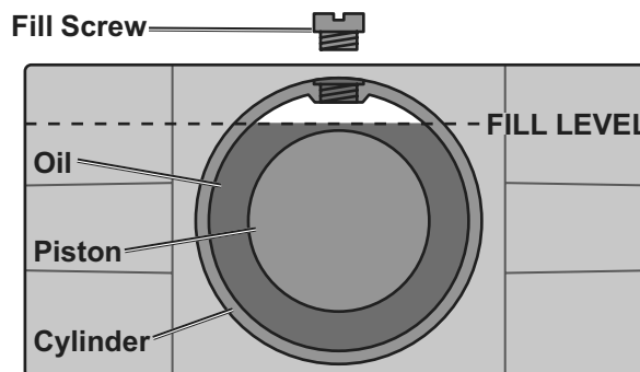
Figure C: Fill Level
