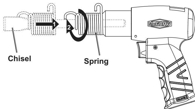
Figure C: Chisel Installation - To twist the Spring on, twist from the hook at the front .
