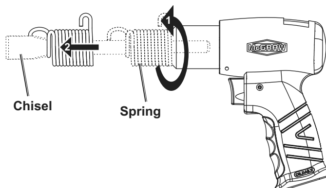
Figure D: Chisel Removal - To twist the Spring off, twist from the hook at the back .
