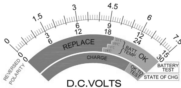
Volts Gauge
