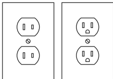
Figure A: Outlets for 2-Prong Plug
