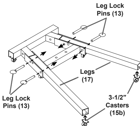
Figure B: Attach Legs
