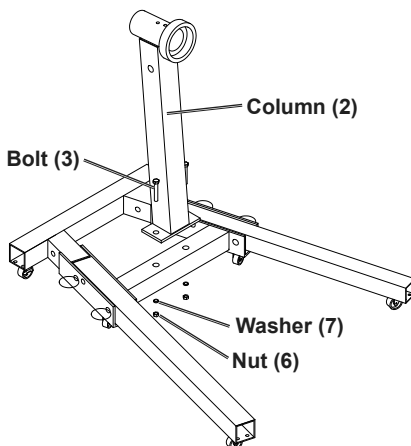
Figure C: Attach Column
