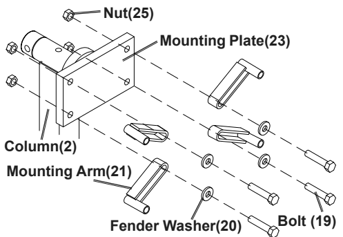
Figure F: Attach Mounting Arm
