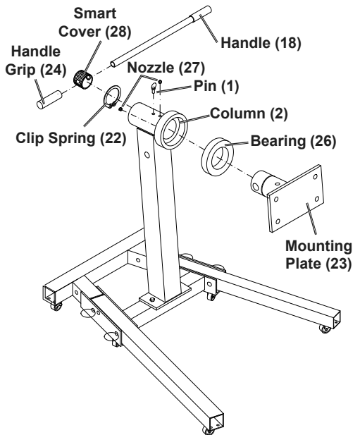
Figure E: Attach Mounting Plate
