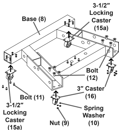
Figure A: Attach Casters to Base
