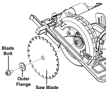
Figure A: Blade Installation
