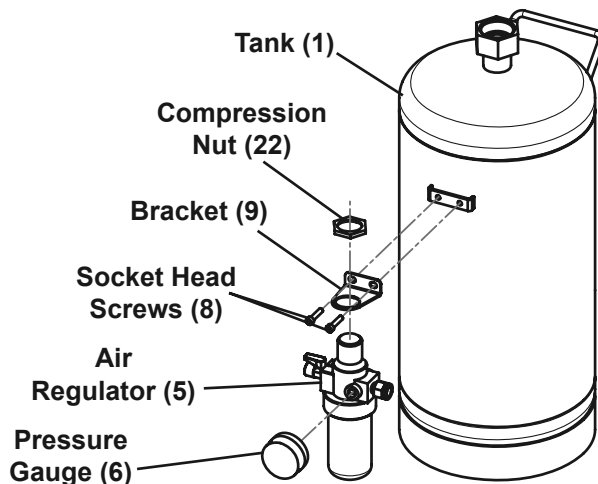
Figure A: Air Regulator Assembly
