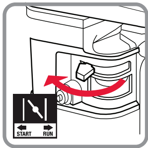
1. CLOSE CHOKE
