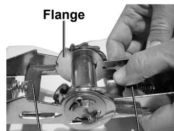
Release Tab A Release Tab B Figure D: Releasing the Strap
