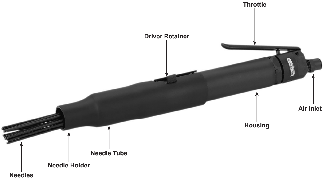
Air Needle Scaler Components
