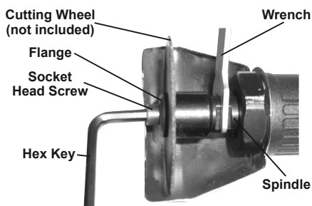
Figure C: Attaching Cutting Wheel
