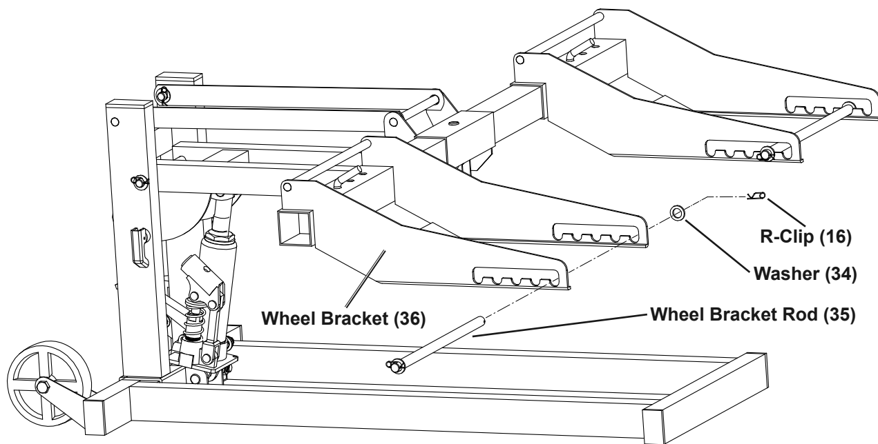
Step 6: Attach Wheel Bracket Rods
