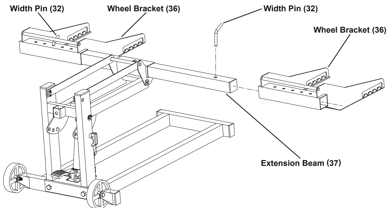
Step 5: Install Wheel Brackets
