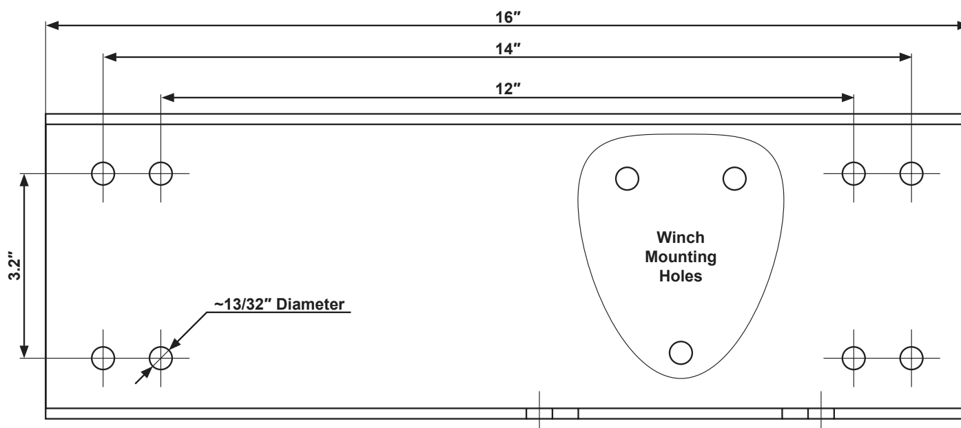
Figure A: Mounting Hole Diagram
