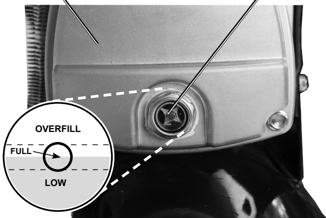
Figure D: Oil Sight Gauge
