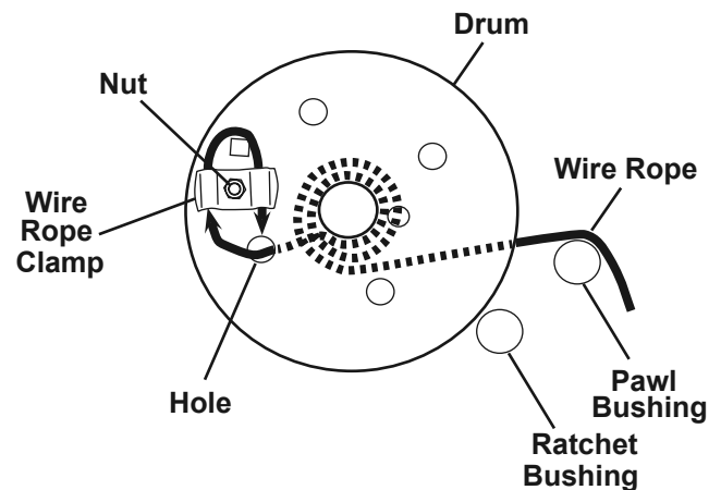
Figure G: : Wire Rope Replacement
