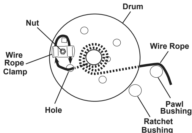
Figure G: : Wire Rope Replacement
