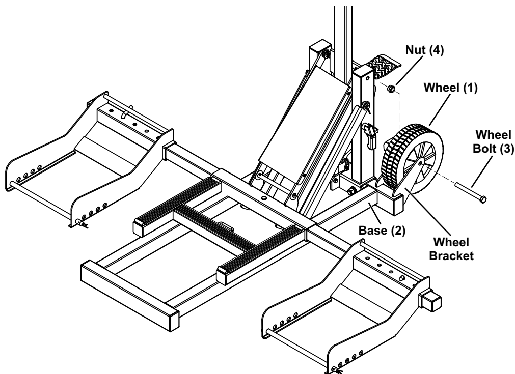
Step 8: Attach Wheels
