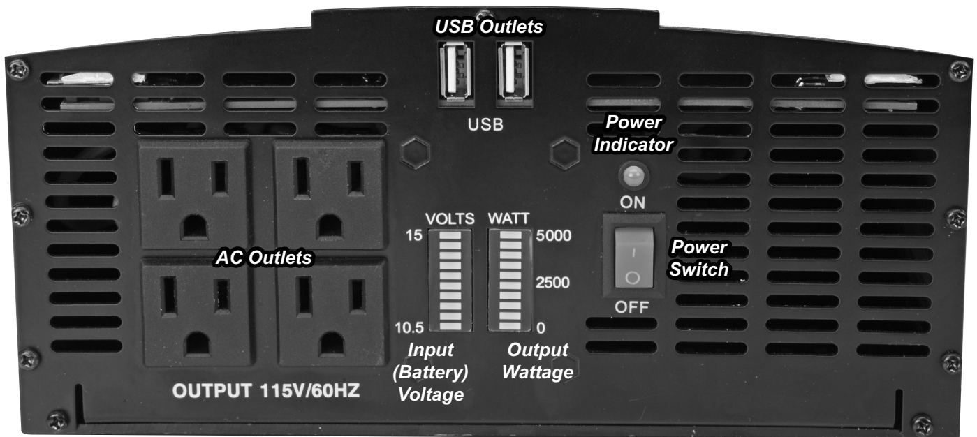
Figure B: Control Panel Components
