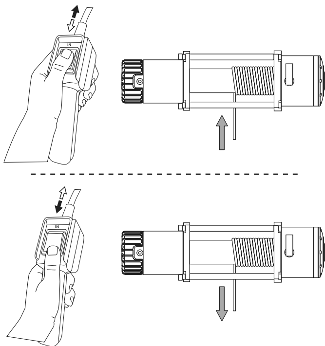
Figure L: Pendant controls
