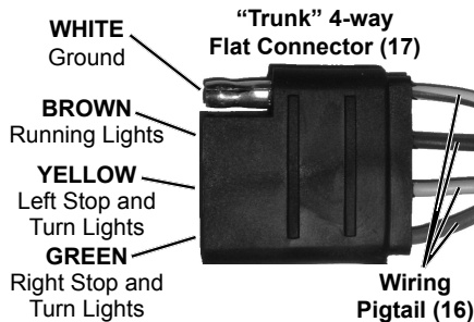
Figure A: Wiring Color Code
