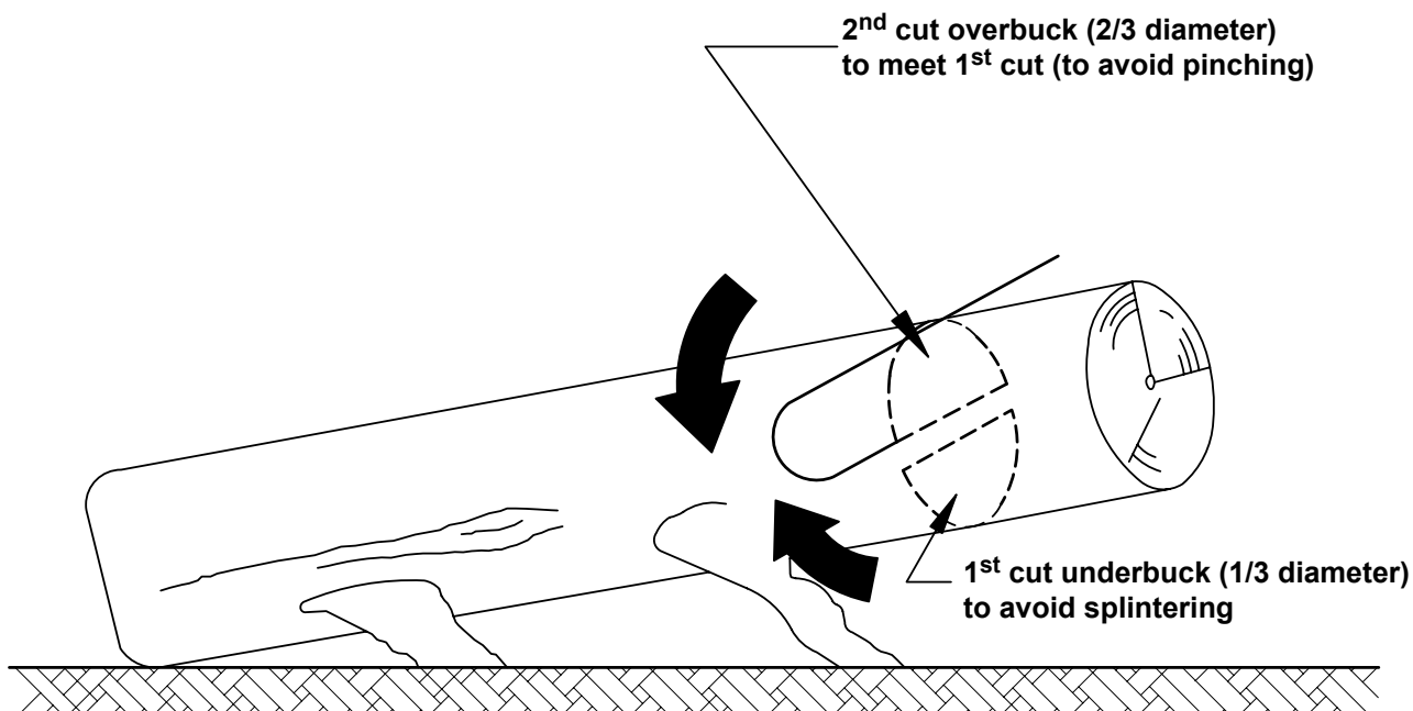
Figure N: Log Supported One End
