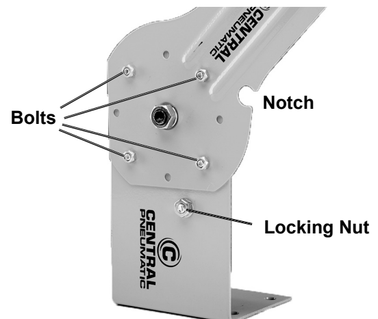
Figure A: Adjusting the Guide Roller Bracket.
