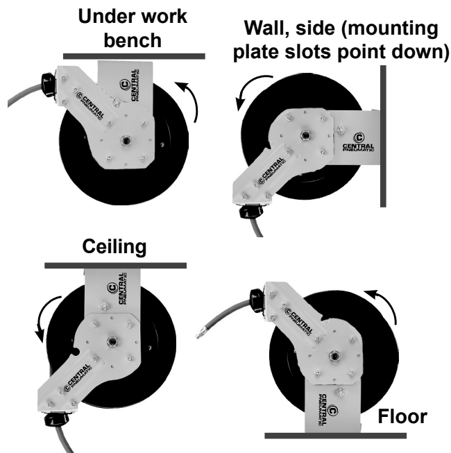
Figure C: Mounting examples.
