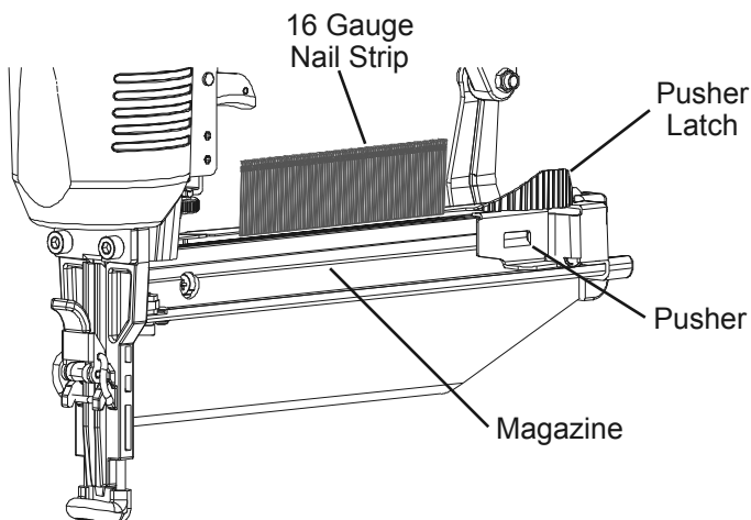
Figure C: Nail Loading Detail
