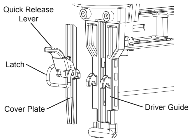
Figure D: Driver Guide and Cover Plate Detail
