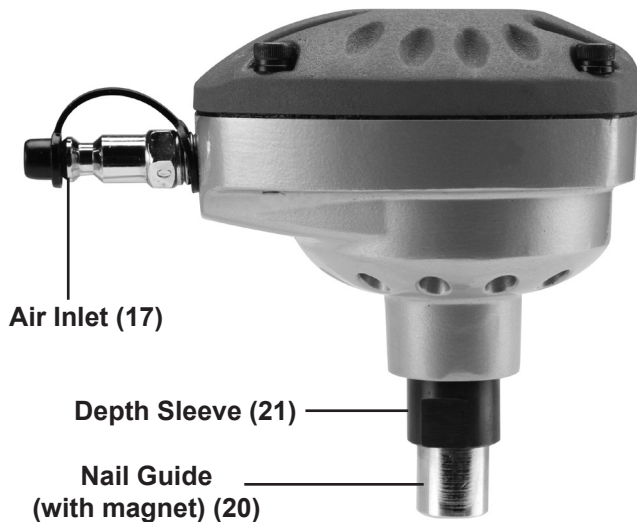
Figure A: Components and Controls
