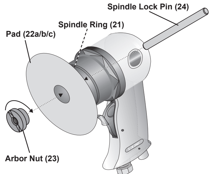
Figure D: Installing the Pad
