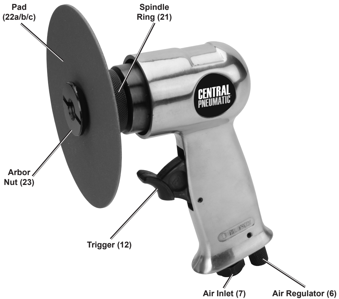
Figure A: Components and Controls
