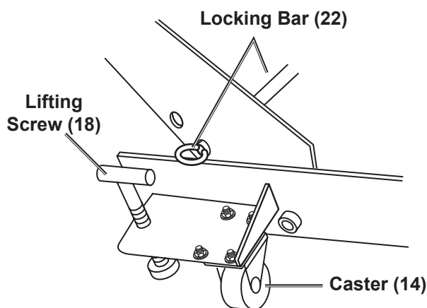
Figure A: Lifting Screw and Locking Bar
