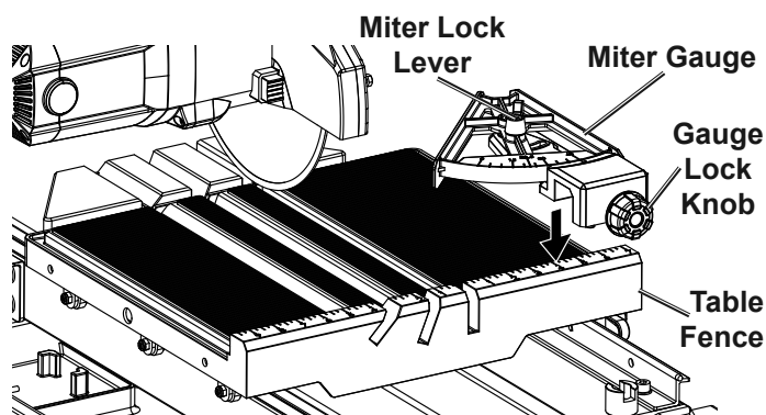
Figure K: Miter Gauge
