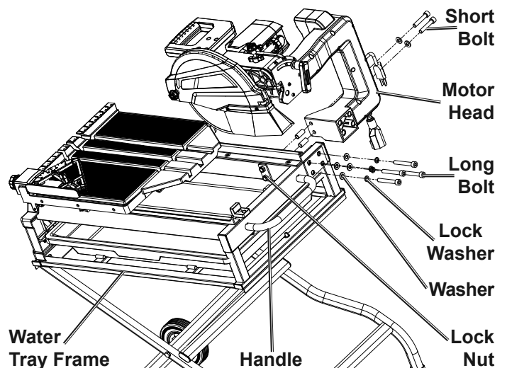
Figure E: Motor Head Installation
