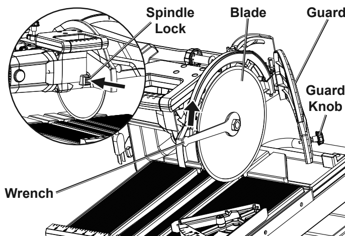
Figure J: Securing Blade
