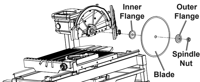
Figure I: Blade Assembly
