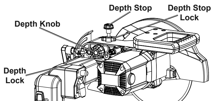
Figure M: Depth Controls
