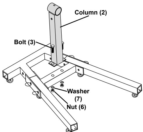
Figure C: Attach Column
