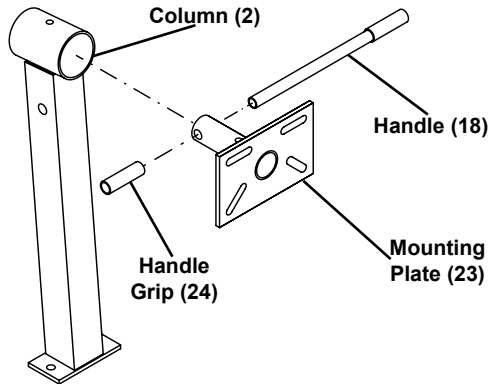
Figure E: Attach Mounting Plate
