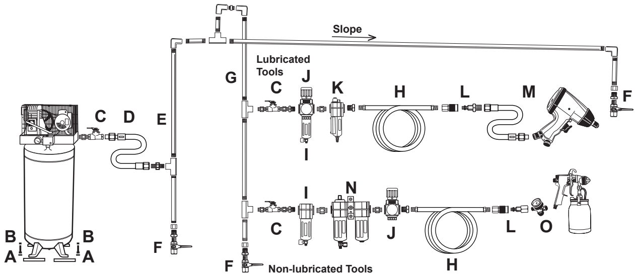
Figure C: Stationary Air Supply Setup
