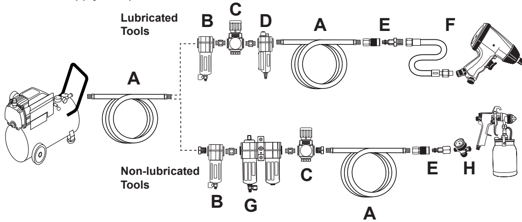
Figure B: Portable Air Supply Setup
