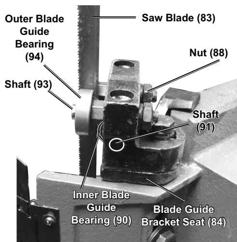
Figure Q: Lower Blade Guide Assembly
