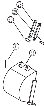
Figure B (Taken from Assembly Diagram from 93167 Trencher manual.)
